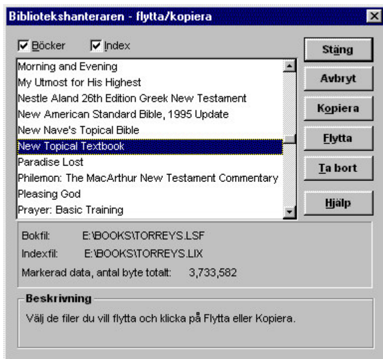
Figure 7-14 Dialogrutan Bibliotekshanteraren.
